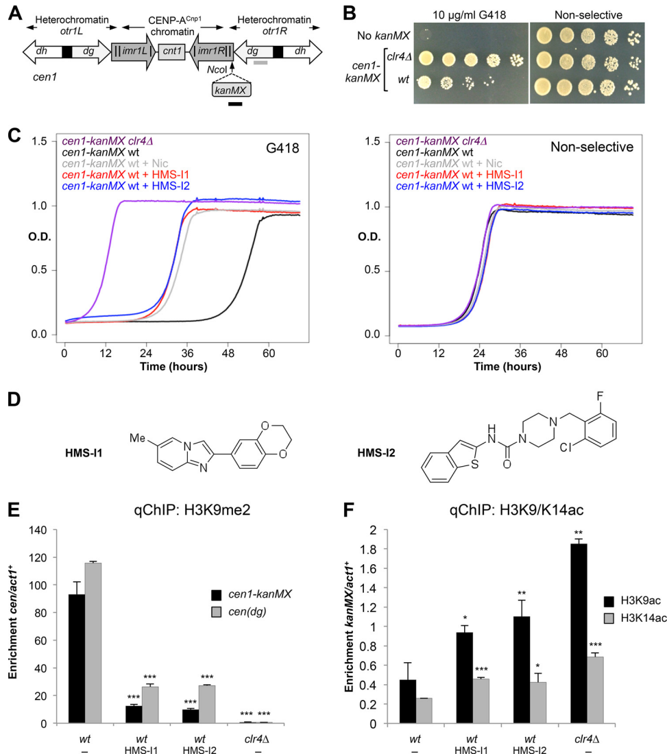
FIG 1 HMS-I1 and HMS-I2 disrupt centromeric heterochromatin integrity in fission yeast. (A) Schematic diagram showing the position of the cen1 imr1R(Nco1):kanMX ( cen1-kanMX for short) reporter gene in centromere 1 relative to the dg and dh outer repeat ( otr ) elements, the innermost repeats ( imr ) and the central core ( cnt ). The position of heterochromatin and CENP-A Cnp1 chromatin domains is indicated. Locations of primers used in panel E below are indicated by the gray and black bars. cen(dg) primers amplify a sequence present in all centromeres. (B) Plating assay of the cen1-kanMX strain on YES plates with 10 μg/ml G418 or without G418 (nonselective). (C) Growth curves of cen1-kanMX cells in YES media with 5 μM HMS-I1, 5 μM HMS-I2, and 10 mM nicotinamide (Nic), with 10 μg/ml G418 or without G418 (nonselective). (D) Chemical structures of HMS-I1 and HMS-I2. (E) qChIP analysis of H3K9me2 levels associated with the cen1-kanMX insertion or cen(dg) repeats, relative to act1 + . (F) qChIP analysis of H3K9ac and H3K14ac levels associated with the cen1-kanMX insertion, relative to act1 + . In panels E and F, cells were grown in media containing 5 μM HMS-I1 and 5 μM HMS-I2, with 10 μg/ml G418. Error bars indicate standard deviations for three biological replicates. *, P < 0.05; **, P < 0.01; ***, P < 0.0001.
