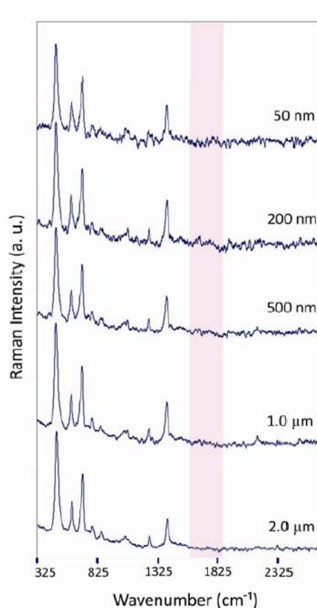
Fig S3. Total Raman spectra of a negatively charged PDMS piece contact-charged against another PDMS piece. The region shaded in pink contains peaks at 1642 cm -1 and 1710-1730 cm -1 (SiCH 2 COOH) and between 1730-1830 cm -1 (RCOOH and RCOOOH, where R=Si or C) characteristic of compositional changes due to contact electrification. The intensity of these peaks decreases as the scan depth is increased from 50 nm to 2.0 μm, confirming that contact-electrification affects predominantly the layer of the material near the surface – this observation agrees with multiple other studies on contact-electrification (16-19).
