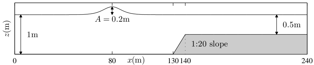
Figure 7: Definition sketch for the submerged shelf reversibility check.
