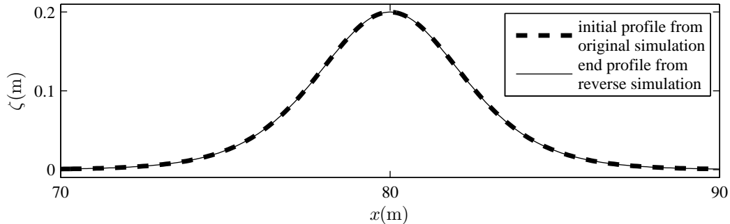
Figure 10: Reversibility comparison - end profile of the reversed simulation superimposed on the initial condition of the original simulation.
