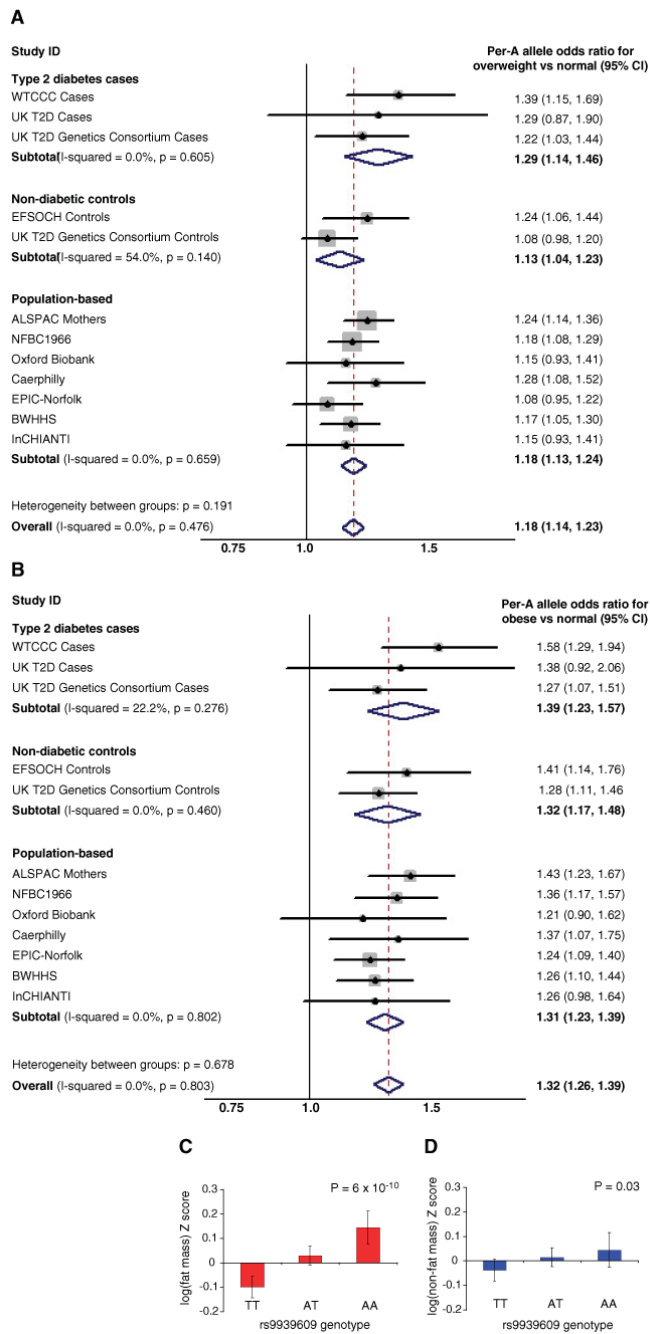
Fig. 2. (A and B) Meta-analysis plots for odds of (A) overweight and (B) obesity, compared with normal weight in adults for each copy of the A allele of rs9939609 carried. (C and D) Bar charts showing (C) DEXA-measured fat mass in 9-year-old children and (D) DEXA-measured lean mass in 9-year-old children, both from the ALSPAC study. Error bars represent 95% confidence intervals
