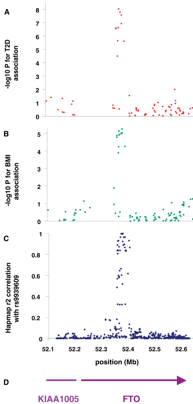
Fig. 1. Associations of SNPs in the FTO/KIAA1005 region of chromosome 16 with (A) type 2 diabetes using 1924 cases and 2938 controls and (B) adult BMI in type 2 diabetic patients. (C) Linkage disequilibrium ( r^2 ) between associated SNP rs9939609 and all other SNPs in HapMap data in Caucasian European samples. (D) Gene positions.
