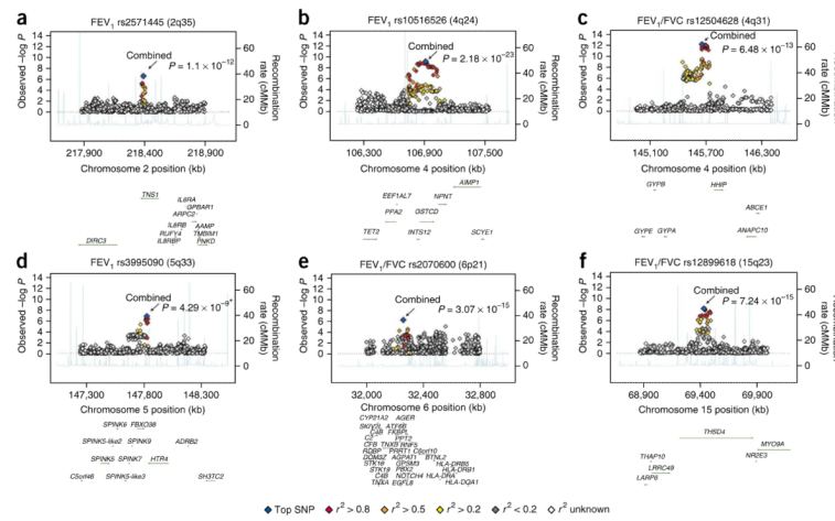
Figure 2. Regional association plots of six lung function–associated loci. (a–f) Statistical significance of each SNP on the -\log_{10} scale as a function of chromosome position (NCBI build 36) in the meta-analysis of stage 1 data alone. The sentinel SNP at each locus is shown in blue; the correlations ( r^2 ) of each of the surrounding SNPs to the sentinel SNP are shown in the indicated colors. The six loci included are those that showed association with FEV 1 or FEV 1 /FVC ( P < 5 \times 10^{-8} ) in the meta-analysis of data from stages 1, 2a and 2b. The combined P values for all stages are indicated by arrows. The relevant trait (FEV 1 or FEV 1 /FVC ratio) is indicated for each plot. For rs12504628, the plot shows only the association of FEV 1 /FVC; this SNP was associated ( P < 5 \times 10^{-8} ) with both FEV 1 and FEV 1 /FVC. Fine-scale recombination rate is plotted in blue 39 . Combined P value from stages 1 and 2a only; SNP rs3995090 had low imputation quality in the CHARGE Consortium data and so was not included in stage 2b.
