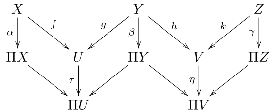
Fig. 5. Composing cospans.
