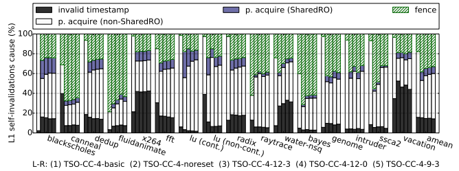
Figure 9. Breakdown of L1 self-invalidation cause.
