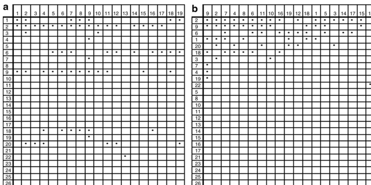
FIG. 1. (a) Example of a J \times K matrix of indicator variables ( J = number of symptoms; K = number of episodes) for subject 6010 with symptoms 1–26 listed vertically and hypoglycemic episodes listed horizontally. Each reported symptom is marked with a square. (b) Rearrangement of the matrix rows and columns so that rows now appear according to the frequency with which symptoms are experienced and columns according to the number of symptoms per episode (both following a descending order from the top-left corner).
