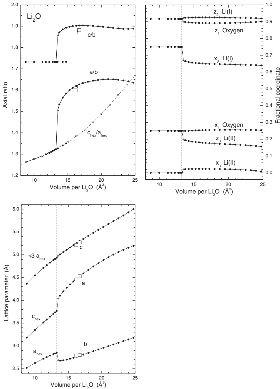
FIG. 3. The evolution under pressure of the lattice constants ( a , b , and c -orthorhombic; a_{hex} and c_{hex} -hexagonal) and the internal structural parameters ( x_1 \cdots z_3 of anticotunnite) of \text{Li}_2\text{O} . Pronounced discontinuities are observed between 13.25 and 13.5 \text{ \AA}^3/\text{Li}_2\text{O} . The solid lines connecting the axial ratio data correspond to the true minima of the total energy while the few isolated solid symbols around 14 \text{ \AA}^3/\text{Li}_2\text{O} were obtained by structural optimization at increasing volumes within a narrow parameter space. Open symbols represent the subset of experimental data from Table I (Refs. 4 and 5).
