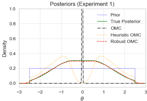
Figure 1: An example where OMC fails to approximate the true posterior, collapsing a region of similar likelihood into a single point. Heuristic OMC is a simple heuristic that (unsuccessfully) attempts to solve this issue. Robust OMC is the approach proposed in this paper. See Subsection 4.1 for details.
