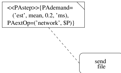
Fig. 19. External operation
