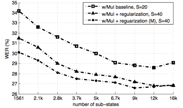
Fig. 5. 5 Hour Training Data Case: WER of cross-lingual systems with and without the original \ell_1 -norm regularization and the modified regularization (M).
