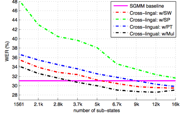
Fig. 4. 5 Hour Training Data Case: WER of cross-lingual systems. In these experiments, the dimension of state vectors is 20. The best performance is achieved by multilingual subspace system denoted as “w/Mul” and the WER is 28.6% which is considerably better than 31.1% by SGMM baseline.
