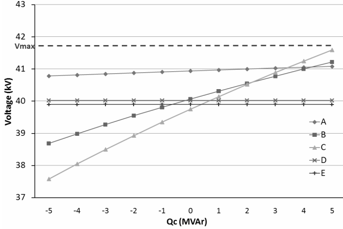
Fig. 3. Voltage sensitivity of all buses to reactive power injections at Bus C (kV/MVAr)
