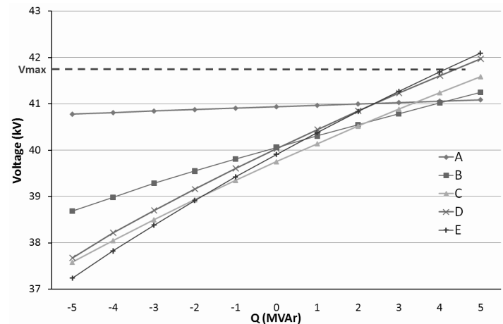
Fig. 2. Individual bus voltage sensitivities to reactive power injections at the same bus (kV/MVar)
