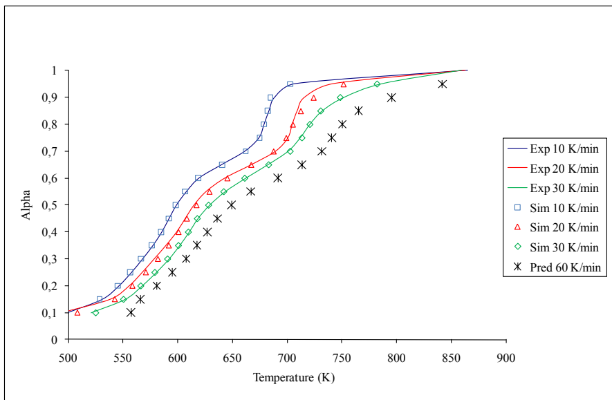
Fig. 7: Experimental (lines) and simulated (symbols) curves of conversion degree vs. temperature at different heating rates for sample Sib 2
