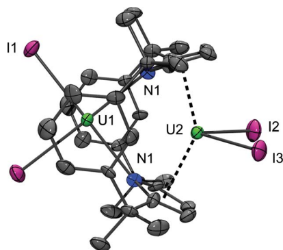
Fig. 3 Solid state structure of 4 (displacement ellipsoids are drawn at 50% probability). For clarity, H atoms are omitted. Selected bond distances (Å) and angles ( ^\circ ) for 4 : \text{U1-I1} 3.1096(6) , \text{U1-N1} 2.669(5) , \text{U1}-[\text{aryl1}]_{\text{cent(ave)}} 2.799 , \text{U1}-[\text{aryl2}]_{\text{cent(ave)}} 2.748 , \text{U1-C}_{\text{avg}} 3.105 , \text{C-C} 1.383(9) – 1.410(8) , \text{U2-C}_{\text{avg}} 2.869 , [\text{aryl1}]_{\text{cent}}\text{-U1}-[\text{aryl2}]_{\text{cent}} 164.99 , \text{U2-I2} 3.0432(8) , \text{U2-I3} 3.0256(8) , \text{U2}-[\kappa^5\text{-C}_4\text{N}]_{\text{cent(ave)}} 2.583 , [\kappa^5\text{-C}_4\text{N}]_{\text{cent}}\text{-U2}-[\kappa^5\text{-C}_4\text{N}]_{\text{cent}} 139.03 , \text{U1}\cdots\text{U2} 3.8639(5) .
