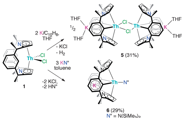
Scheme 6 Syntheses of [\text{K}(\text{THF})_2\text{Th}(\mu\text{-Cl})(\text{L}^{-2\text{H}})]_2 , 5 and [\text{Th}(\text{N}'')(\text{L}^{-2\text{H}})] , 6 .
