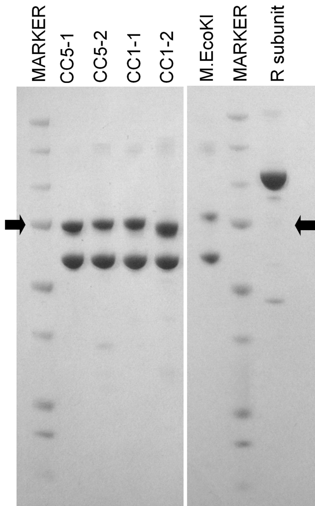
Figure 2. SDS-PAGE analysis of purified proteins. The upper band in the MTase preparations is the EGFP-His-tagged S subunit and the lower band is the M subunit. The EcoKI MTase with the EGFP-His-tagged S subunit is shown for comparison. The purified R subunit is also shown. The markers have molecular masses of 250, 150, 100, 75, 50, 37, 25 and 20 kDa (Biorad precision plus protein standards). The arrows indicate the 75 kDa size.
