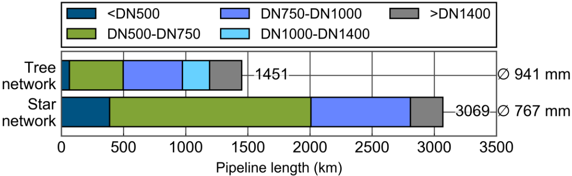
Figure 14. Comparison of the pipeline lengths of the two different networks considered.
