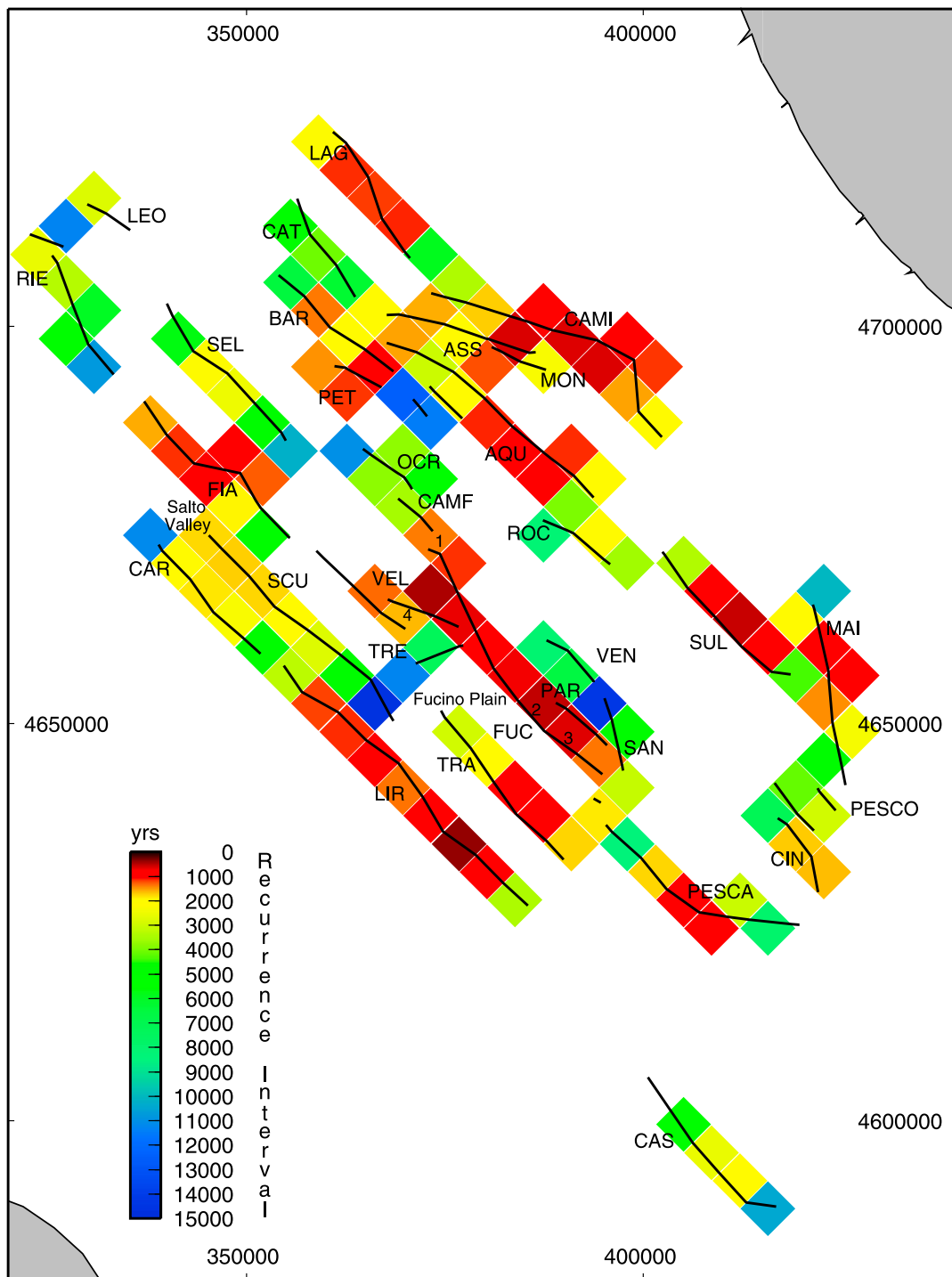
Figure 8. Map showing spatial distribution of earthquake recurrence intervals at a 5 \text{ km} \times 5 \text{ km} resolution calculated from Late Pleistocene-Holocene offsets and assuming all earthquakes are dip-slip events with 1 m of slip. Grid squares containing discussed published paleoseismic observations are shown: 1, Pantosti et al. [1996]; 2, Michetti et al. [1996]; 3, Galadini and Galli [1999]; 4, Palumbo et al. [2004]. AQU = L'Aquila Fault, ASS = Assergi Fault, BAR = Barete Fault, CAMF = Campo Felice Fault, CAMI = Campo Imperatore Fault, CAR = Carsoli Fault, CAS = Cassino Fault, CAT = Capitignano Fault, CIN = Cinque Miglia-Aremogna Fault, FIA = Fiamignano Fault, FUC = Fucino Fault, LEO = Leonessa Fault, LAG = Laga Fault, LIR = Liri Fault, MAI = Maiella Fault, MON = Monte Christo Fault, OCR = Ocre Fault, PAR = Parasano-Pescina Fault, PESCA = Pescasseroli Fault, PESCO = Pescocostanzo Fault, PET = Pettino Fault, RIE = Rieti Fault, ROC = Roccapreturo Fault, SAN = San Sebastiano Fault, SCU = Scurcola Fault, SEL = Sella di Corno Fault, TRA = Trassaco Fault, TRE = Tre Monti Fault, VEL = Velino-Magnola Fault, VEN = Ventrino Fault.
