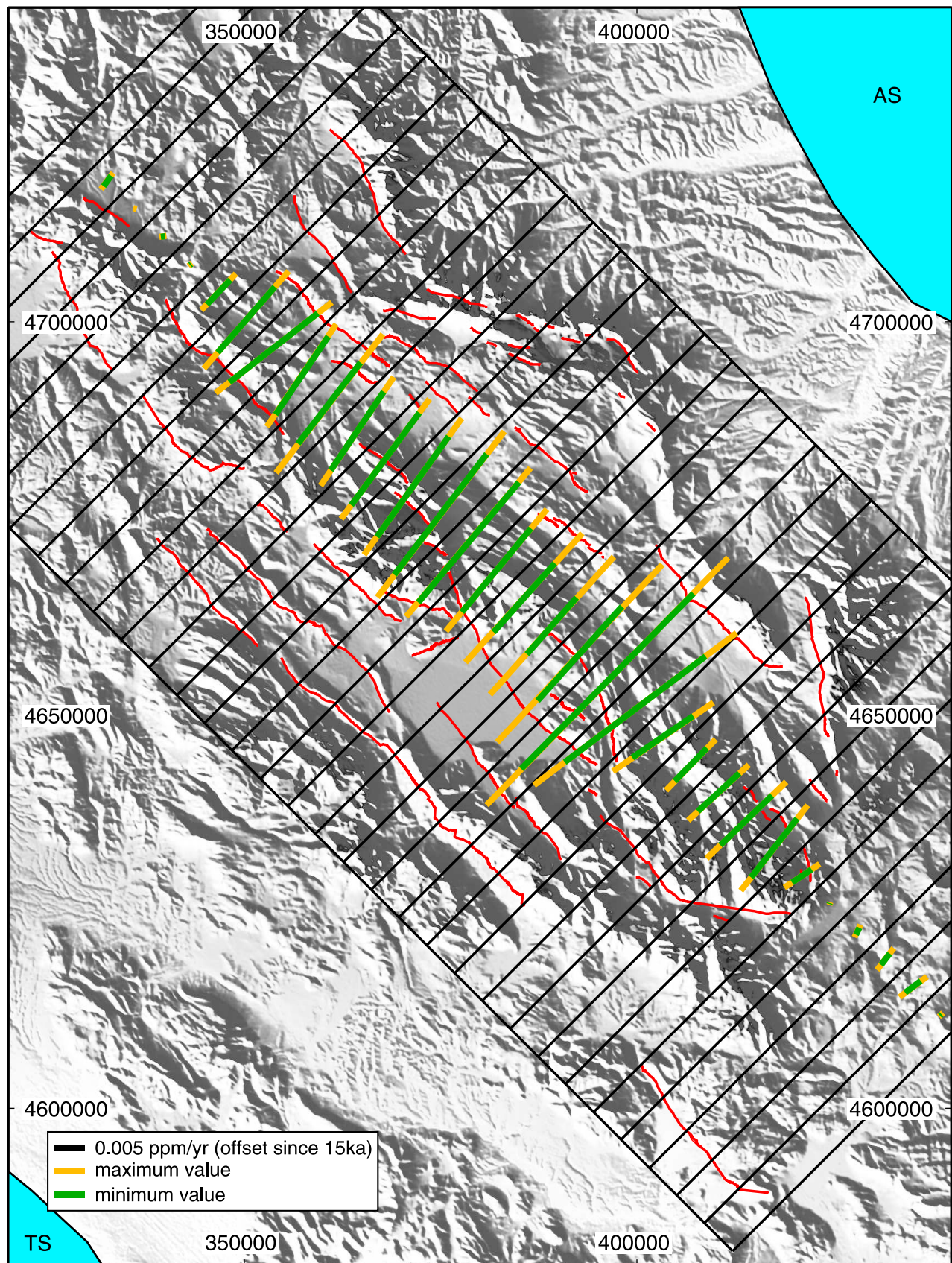
Figure 5. Principal horizontal strain-rates and extension rates along 5 \text{ km} \times 80 \text{ km} transects across the Apennines calculated from offsets of Late Pleistocene-Holocene landforms showing how they change along the axis of the chain from NW to SE. AS = Adriatic Sea, TS = Tyrrhenian Sea.
