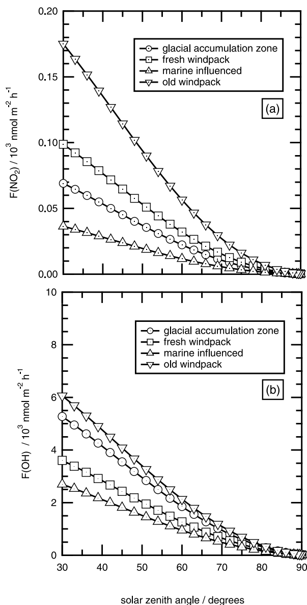
Figure 4. Calculated depth-integrated production rates (fluxes) versus solar zenith angle for clear-sky conditions for each of the four snowpacks studied near Ny-Ålesund. (a) Depth-integrated production rate (flux) of NO 2 from nitrate photolysis calculated using values of nitrate recorded in Table 1. (b) Depth-integrated production rate of OH radicals from hydrogen peroxide photolysis, assuming a concentration of 4 \mu\text{mol l}^{-1} of H 2 O 2 .
