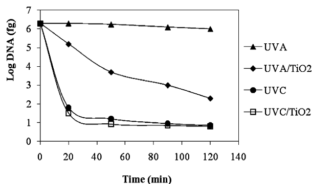
Fig. 6 Detection of E. coli genomic DNA in 0.8% (w/v) NaCl aqueous solution during its treatment by UV-A/TiO 2 ; [TiO 2 ] = 200 mg L -1 , UV-A alone, UV-C alone and UV-C/TiO 2 ; [TiO 2 ] = 25 mg L -1 by the real-time qPCR assay.
