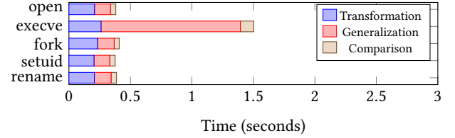
Figure 5. Timing results: SPADE+Graphviz
