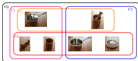
Figure 1: Null counting context c_0 and disjoint counting contexts c_1 - c_4
