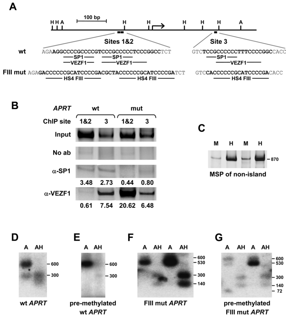
Figure 8. VEZF1 elements protect a CpG island from de novo DNA methylation. (A) Scale representation of the 700 bp hamster APRT CpG island (CGI). The positions of AvalI (A) and HpaII (H) restriction sites are indicated. The locations of putative SP1 and VEZF1 binding motifs in the wild type (wt) sequence are shown. The sequence alterations in the mutant (mut) are shown beneath, where all three SP1/VEZF1 motifs are replaced with the VEZF1-specific footprint III (CCCCCGCATCCCCGA) sequence from the HS4 insulator. (B) ChIP analysis of SP1 and VEZF1 interactions with stably integrated hamster APRT CGI sequences in mouse ES cells. PCR primers flanking either sites 1 and 2 (1&2) or site 3 were used to detect interactions with either the wild type (wt) APRT CGI or the mutant (FIII mut) containing VEZF1-specific sites. PCR products shown are ~180 bp in size. DNA enrichments relative to input and normalized to no antibody control are shown. (C) Methylation specific PCR (MSP) analysis of a stably integrated non-island region of the APRT locus. Genomic DNA was digested with either of the isoschizomers MspI (M) or CpG methylation-sensitive HpaII (H), followed by PCR over the CpG-containing sites. Increased PCR product from HpaII relative to MspI digested DNA demonstrates the presence of de novo methylation at these sites in ES cells. Two representative lines are shown. (D–G) VEZF1 sites are sufficient for the demethylation of the APRT CpG island. Southern blotting of APRT CpG island elements stably integrated into ES cells. Genomic DNA was digested with AvalI alone (A) or with AvalI and HpaII (AH). Digestion of the ~600 bp AvalI parent fragments with HpaII indicates the absence of DNA methylation. (D,E) Representative lines harboring the wild type APRT CGI that was unmethylated or in vitro methylated with M.SssI prior to integration. (F,G) Two representative lines harboring the mutant APRT CGI, whose SP1 motifs are substituted with VEZF1-specific FIII sites from HS4, that were unmethylated or pre-methylated prior to integration.
