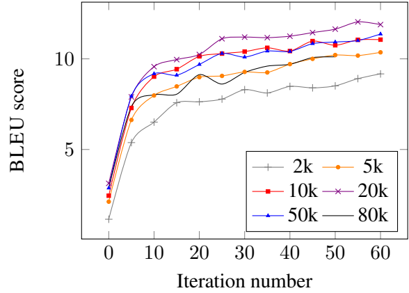
Figure 1: The effect of the number of subword operations on BLEU score during training for \text{EN} \rightarrow \text{GU} (calculated on the newsdev2019 dataset).
