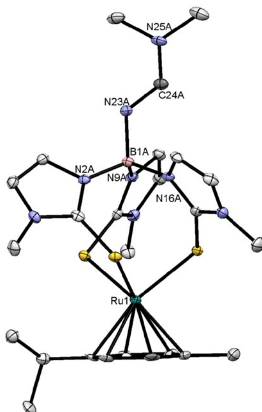
Figure 9: Structure of the dication in [ \kappa^3 -[S,S,S]- (N,N-dimethylformamidine)B(methimazoly)] 3 Ru(p-cymene)][PF 6 ] 2 ( 12 ). Hydrogen atoms, counter-ions and MeCN solvent omitted for clarity. Selected bond lengths and angles are provided in Table 1 .
