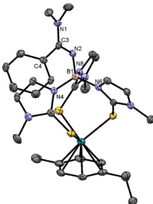
Figure 5. Structure of the dication in [ \kappa^3 -[S,S,S]-(N,N-dimethylbenzimidine)B(methimazolyl) 3 Ru( p -cymene)] 2+ [PF 6 ] 2 ( 7 ). Hydrogen atoms, counter-ions and MeCN solvent omitted for clarity. Selected bond lengths and angles are provided in Table 1.
