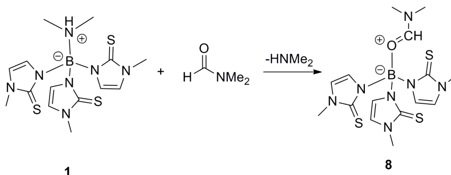
Scheme 4. Direct route to (DMF)ZTm ( 8 ).
