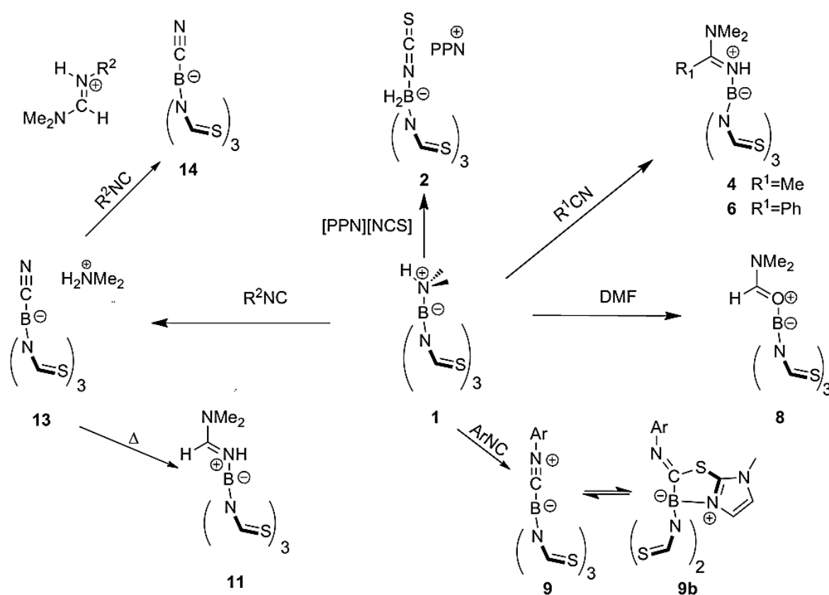
Scheme 9. Reactions of 1 described in this work. R^1 = \text{Me, Ph} ; Ar = 2,6\text{-dimethylphenyl} ; R^2 = 1,1\text{-3,3-dimethylbutyl} .
