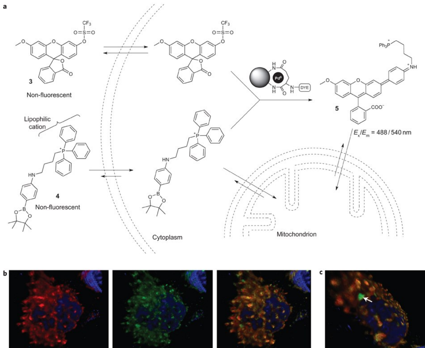
Figure 3. a , \text{Pd}^0 -catalysed intracellular cross-coupling of reagents 3 and 4 generates the mitochondria-localized fluorescent compound 5 . b,c , HeLa cells were loaded with \text{Pd}^0 microspheres, washed to eliminate extracellular \text{Pd}^0 microspheres, and subsequently incubated for 48 h with reagents 3 and 4 . Cells were incubated for 30 min with MitoTracker Deep Red (mitochondrial stain), fixed with paraformaldehyde, incubated with Hoechst 33342 (nuclei stain) and imaged by confocal microscopy. Deconvolved confocal images ( b ) of a single cell showing co-localization of MitoTracker-labelled mitochondria and Suzuki–Miyaura product 5 . Left panel: cell nucleus (blue) and mitochondria (red). Centre panel: cell nucleus (blue) and in cellulo synthesized compound 5 (green). Right panel: merged image (orange indicates co-localization). Merged image ( c ) of the same cell observed from a different angle. White arrow indicates the presence of a Texas Red-labelled \text{Pd}^0 microsphere (not localized within the mitochondria), which was imaged using a 550/20 nm emission filter together with compound 5 .
