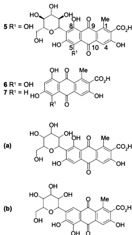
Figure 2. The characteristic constituents observed in the acid hydrolysed extracts of Mexican cochineal ( Dactylopius coccus Costa) dyed yarns together with the proposed structures for the unknown dcII (the stereochemistry of the sugar moieties are currently unknown).
